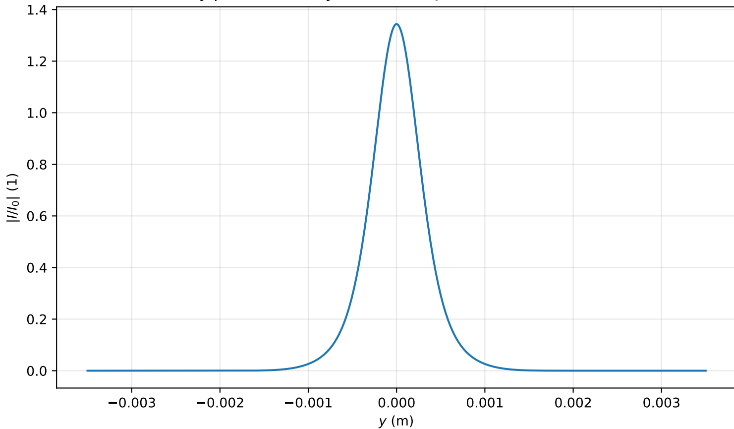
Intensity profile I(x=0, y, z=1.274)/I_0 , P_{in}=0.8P_{cr} , artificial time
